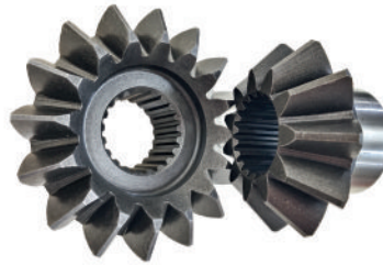
Crown Pinion 11T (19S) x 16T (21S) Part No. NR 2752
