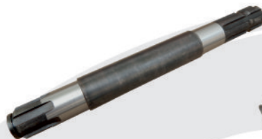
Input Shaft 6Tx6T Part No. NR 3151
