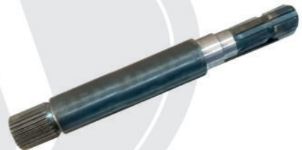
Output Shaft Multi Speed (6Tx10T) (9no Bearing ,307mm ) Part No. NR 004
