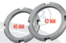
Check Nut 40 MM Round | Part No. NR 1085 Check Nut 42 MM Round | Part No. NR 1086 Check Nut 50 MM Round | Part No. NR 1087
