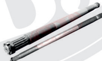
Jack Shaft 35"/6ft. (14Tx14T) 892mm (8 No. Brg) Part No. NR 6619
