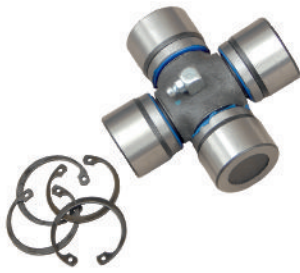
UJ Cross Suitable For Maschio with Outer Locks (35x94mm)
