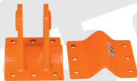
Clevis Bracket Part No. NR 854 (W/Paint) Clevis Bracket Part No. NR 6886 (W/out Paint)
