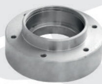
RD Housing 6309 (100mm) (6 Hole) Part No. NR 321
